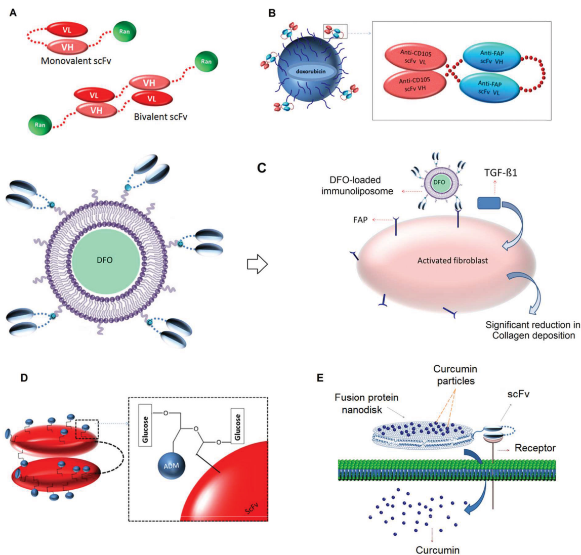
Figure 3. Structure and/or functional mechanism of some scFv-based drug carriers. (A) Monovalent and bivalent formats of Ranpirtase-scFv fusion peptide. Ranpirtase and scFv are joined together with a linker peptide. (B) Schematic view of a doxorubicin-loaded bi-specific IL. The targeting ligand is a fusion peptide composed two scFv molecules, anti-FAP scFv and anti-CD105 scFv. (C) Deferoxamine (DFO)-loaded anti-FAP IL. Anti-FAP scFvs contain a cysteine residue in their linker region that makes a covalent bond with PEG molecules on the surface of liposomes. The resultant ILs are able to bind FAP proteins expressed on the surface of TGF \beta 1-activated fibroblasts and reduce collagen deposition. (D) Adriamycin (ADM)-loaded scFv molecule. Dextran can serve as a linker for effectively loading ADM molecules on scFv molecules. (E) A nanodisk composed of reconstituted high-density lipoprotein particles and apo-AI-anti-CD20 scFv fusion peptide to specifically deliver curcumin to CD20-positive non-Hodgkins lymphoma (NHL) cells. The fusion peptide constitutes the protein scaffold of nanodisk and binds NHL cells through its scFv moiety. The structure of nanodisk has been derived from the work of Crosby and colleagues (71).
