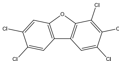
2,3,4,7,8-pentachlorodibenzofuran
