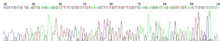
Uncultured Lactobacillus sp. clone BV_LV_OTU6489 16S ribosomal RNA gene, partial sequence Sequence ID: JQ962826.2 Length: 328 Number of Matches: 1
