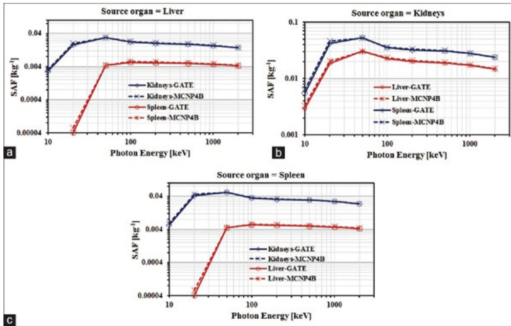
Photon specific absorbed fraction values derived with the GATE and MCNP4B against the photon energy for cross-irradiation from (a) liver, (b) kidneys, and (c) spleen to other selected organs
