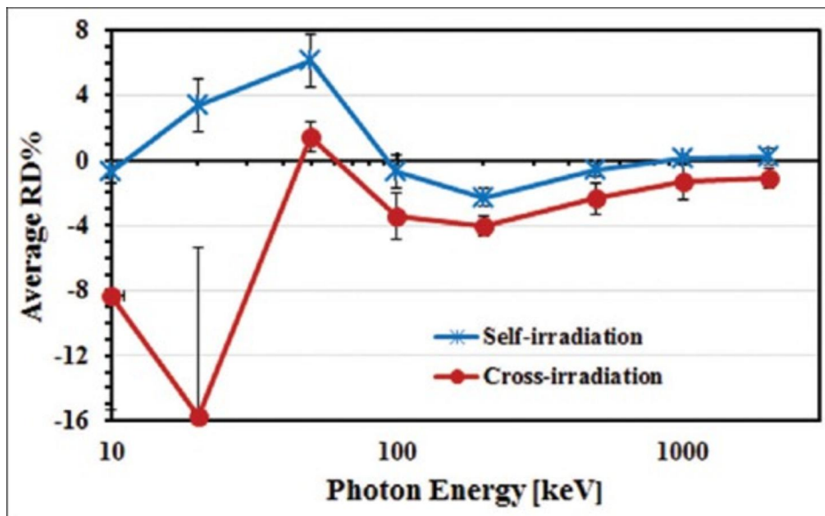
Average of relative percentage difference between the GATE and MCNP4B for self- and cross-irradiation against the photon energy
