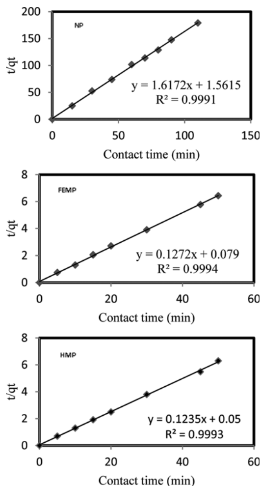
Fig. 5. Pseudo-second-order kinetic sorption of fluoride adsorption.
